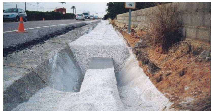
Cuneta filtrante, remontable
